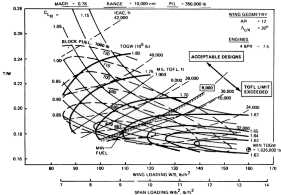
Fig. 3 Engine airframe matching for the reference turbulent airplane.
