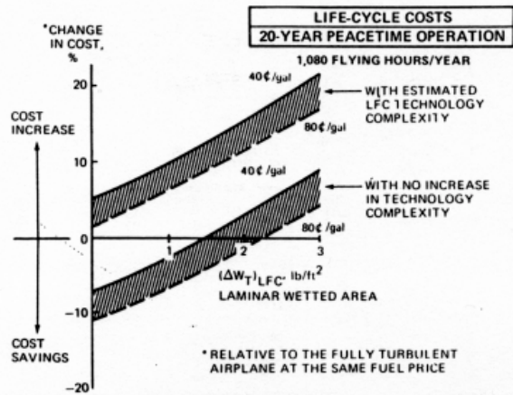
Fig. 13 Effect of technology complexity on relative laminar flow control life-cycle costs.
