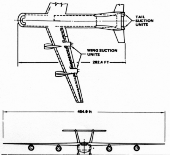
Fig. 8 Final laminar flow control airplane.
