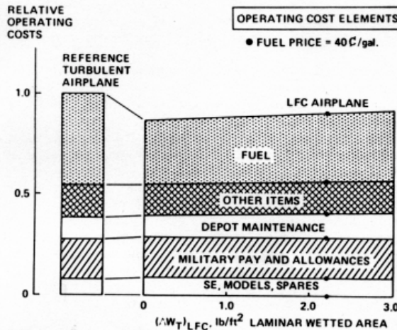
Fig. 12 The 60-day surge conditions cost elements.
