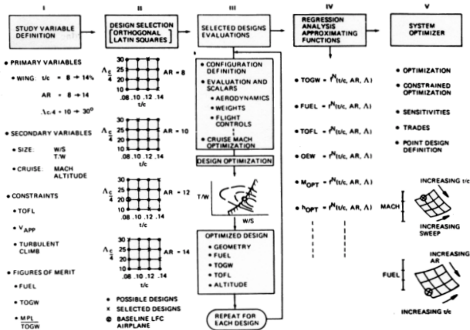
Fig. 4 Laminar flow control wing parametric optimization study.
