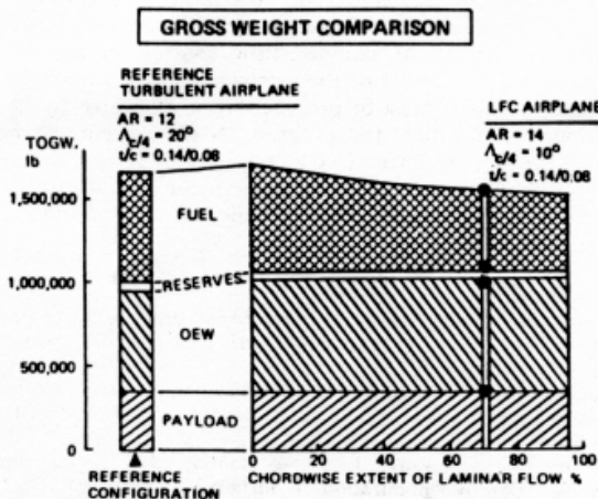
Fig. 9 Laminar flow control fuel and weight savings.
