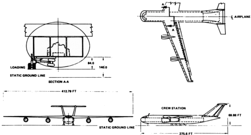
Fig. 2 Reference turbulent airplane.
