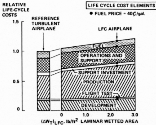
Fig. 11 Twenty-year life cycle cost elements.
