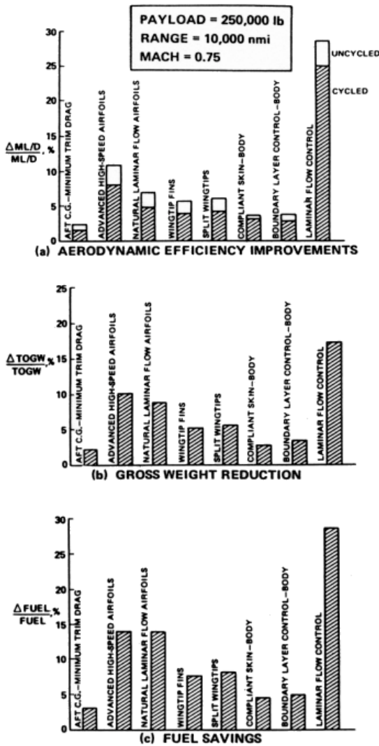
Fig. 1 Potential benefits of advanced aerodynamic concepts.
