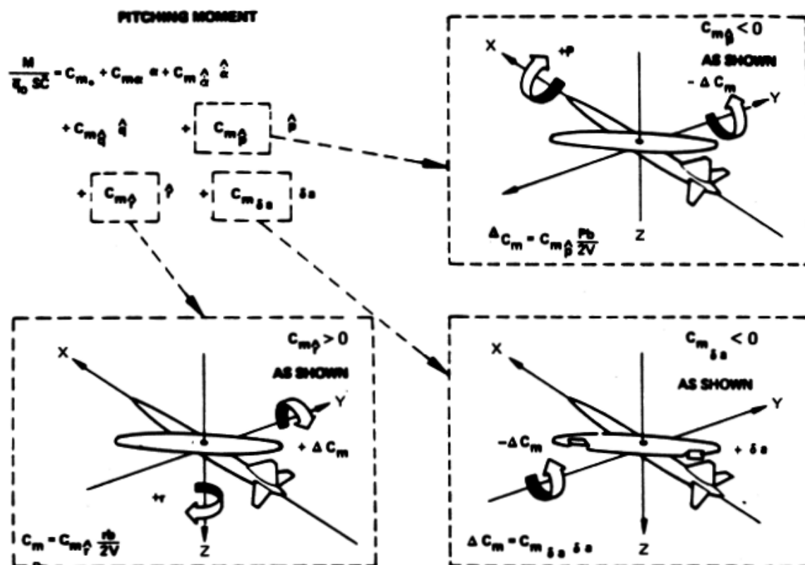
FIGURE 13.—YAWED-WING AERODYNAMIC PITCHING MOMENT CROSS-COUPLING STABILITY DERIVATIVES
