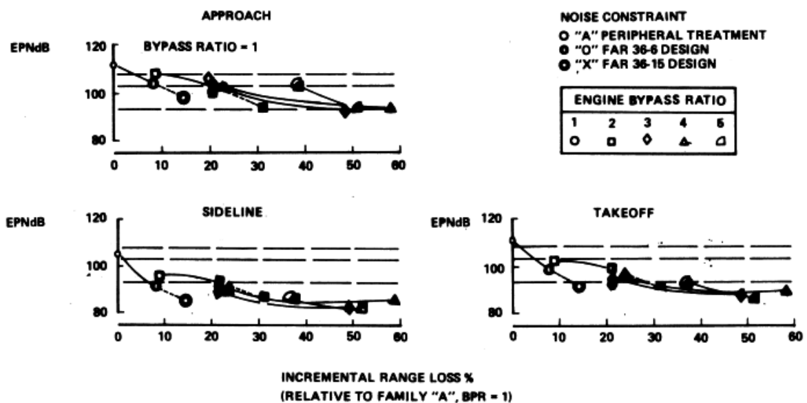
FIGURE 14.—NOISE/PERFORMANCE TRENDS OF "ATT TECHNOLOGY" ENGINES
