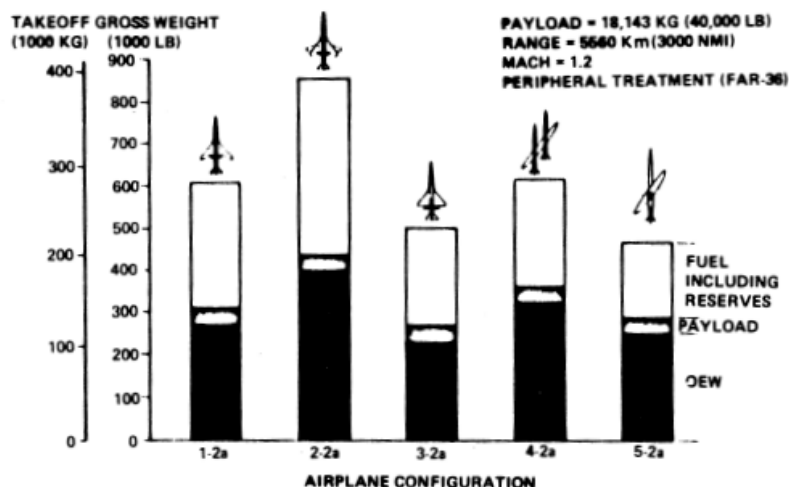
FIGURE 4.—GROSS WEIGHT SUMMARY
