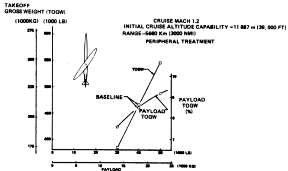
FIGURE 6.—MODEL 5-3A PAYLOAD STUDY
